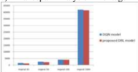
b)Makespan Analysis – Ligo Inspirial
