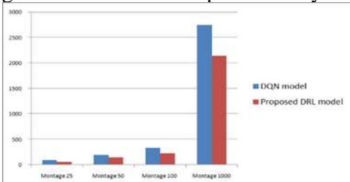
a) Makespan Analysis –Montage
