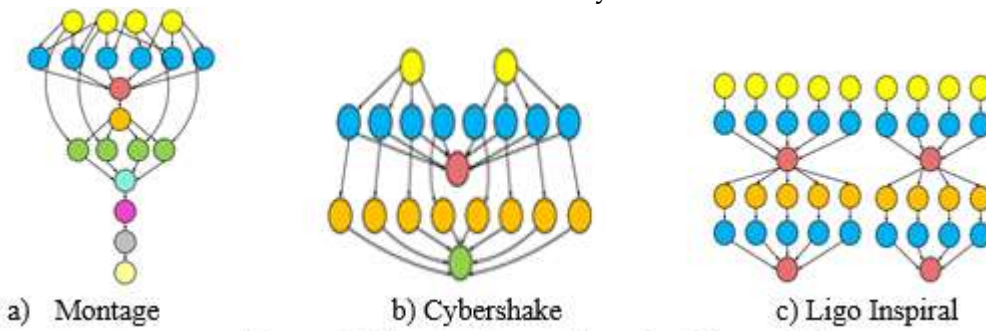
Figure 5. The structure of the scientific workflows
