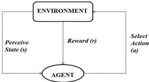
Figure 2. The basic reinforcement learning model
